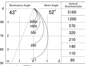
■ Direct Horizontal Illuminance DD161-1050B9035
