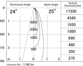
■ Direct Horizontal Illuminance DD161-1025B9040
