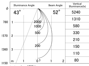
■ Direct Horizontal Illuminance DD161-1050B9040
