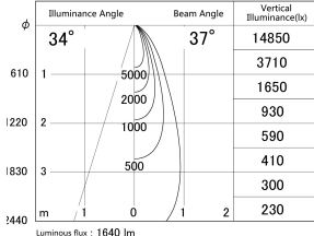
■ Direct Horizontal Illuminance DD161-1535B9040
