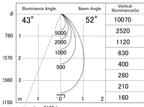
■ Direct Horizontal Illuminance DD161-2050B9040
