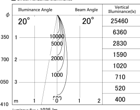
■ Direct Horizontal Illuminance DD161-1020MW9030
