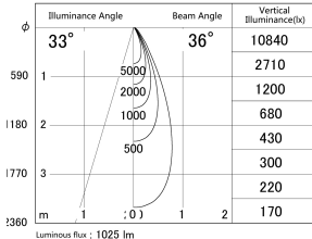
■ Direct Horizontal Illuminance DD161-1035MW9030
