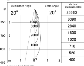
■ Direct Horizontal Illuminance DD161-1020MB9040
