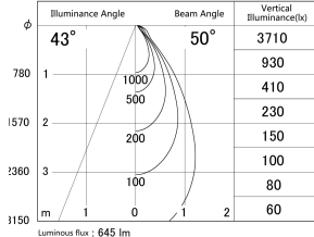
■ Direct Horizontal Illuminance DD161-0845WW9035
