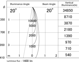
■ Direct Horizontal Illuminance DD161-1520BB9027
