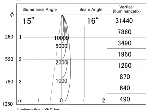
■ Direct Horizontal Illuminance DD161-1015MW9027-TL
