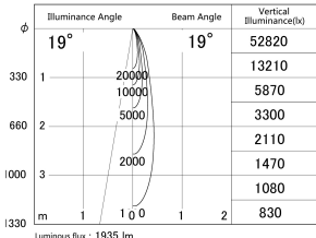
■ Direct Horizontal Illuminance DD161-2520MW9027-TL
