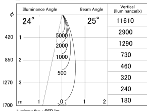
■ Direct Horizontal Illuminance DD161-0825MB9030-TL
