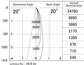
■ Direct Horizontal Illuminance DD161-1520MB9035-TL
