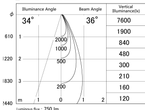
■ Direct Horizontal Illuminance DD161-0835WW9040-TL
