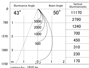
■ Direct Horizontal Illuminance DD161-2545BB9030-TL
