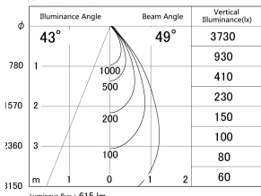
■ Direct Horizontal Illuminance DD161-0845BB9035-TL
