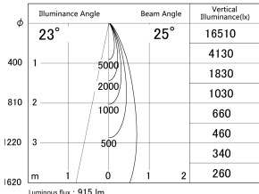
■ Direct Horizontal Illuminance DD161-1025BB9035-TL
