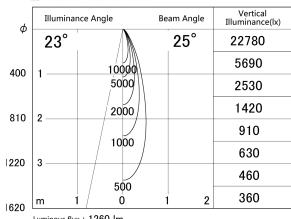
■ Direct Horizontal Illuminance DD161-1525BB9035-TL
