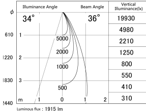
■ Direct Horizontal Illuminance DD161-2035BB9035-TL
