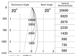
■ Direct Horizontal Illuminance DD161-1520BB9040-TL
