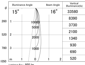
■ Direct Horizontal Illuminance (DD161-1015MW9027-FX)
