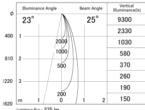
■ Direct Horizontal Illuminance (DD161-0525MW9040-FX)
