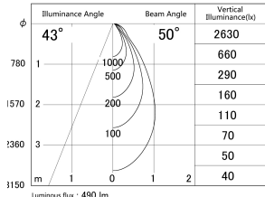
■ Direct Horizontal Illuminance DD161-0545WW9027-FX
