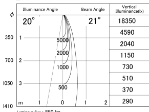
■ Direct Horizontal Illuminance DD161-0820WW9030-FX
