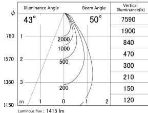
■ Direct Horizontal Illuminance DD161-1545WW9030-FX
