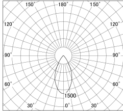
■ Direct Horizontal Illuminance DD161-0845WW9035-FX
