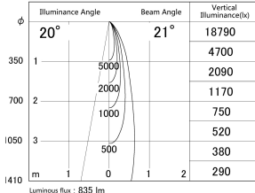
■ Direct Horizontal Illuminance (DD161-0820MW9027-FX-TL)
