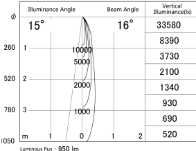
■ Direct Horizontal Illuminance (lx) DD161-1015MW9027-FX-TL
