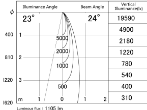
■ Direct Horizontal Illuminance (DD161-1025MW9027-FX-TL)
