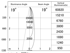
■ Direct Horizontal Illuminance (DD161-2520MW9040-FX-TL)
