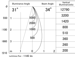
■ Direct Horizontal Illuminance (DD161-1035MB9027-FX-TL)
