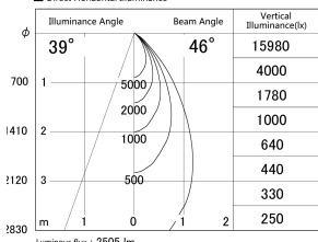
■ Direct Horizontal Illuminance (DD161-2545MB9030-FX-TL)
