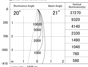
■ Direct Horizontal Illuminance (DD161-1520MB9035-FX-TL)
