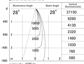
■ Direct Horizontal Illuminance (DD161-2525MB9035-FX-TL)
