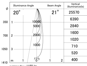
■ Direct Horizontal Illuminance DD161-1020WW9027-FX-TL
