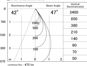
■ Direct Horizontal Illuminance DD130-0550MB9040-DM1
