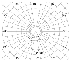
■ Direct Horizontal Illuminance DD130-0550MB9040-DM1
