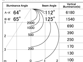
■ Direct Horizontal Illuminance CD026-3460W8050
