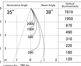
■ Direct Horizontal Illuminance DD146-0835MB9027
