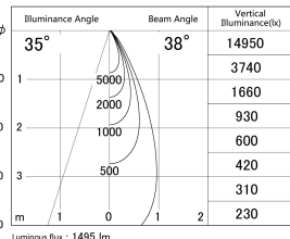
■ Direct Horizontal Illuminance DD146-1535MB9027
