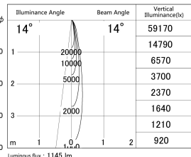
■ Direct Horizontal Illuminance DD146-1515MB9030
