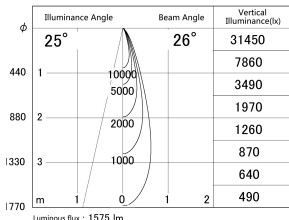
■ Direct Horizontal Illuminance DD146-1525MB9035
