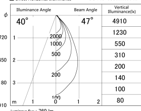
■ Direct Horizontal Illuminance DD146-0850MW9040
