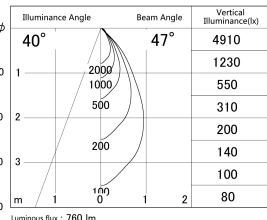
■ Direct Horizontal Illuminance DD146-0850MB9040
