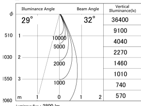
■ Direct Horizontal Illuminance DD146-2535DW9027
