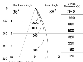
■ Direct Horizontal Illuminance DD146-0835DW9030
