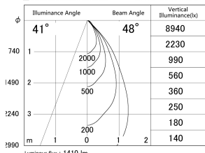
■ Direct Horizontal Illuminance DD146-1550DW9030
