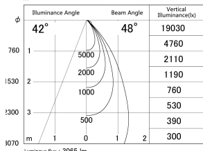
■ Direct Horizontal Illuminance DD146-3050DW9030
