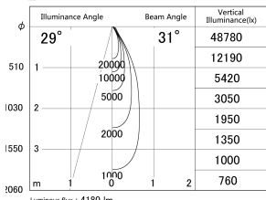
Direct Horizontal Illuminance DD146-4035DW9030
