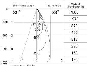
■ Direct Horizontal Illuminance DD146-0835DW9035
